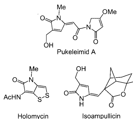
Scheme 1. 5-Alkylidene-2,5-dihydropyrrol-2-one natural products
