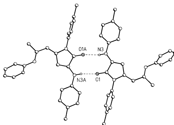
Figure 4. Dimeric structure of 10
