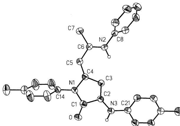
Figure 3. ORTEP plot of 10 . The thermal ellipsoids of 50% probability are shown for the non-hydrogen atoms; selected bond lengths (Å) and angles (°): O–C(1) 1.211(4), N(1)–C(1) 1.368(5), C(2)–C(3) 1.352(5), C(3)–C(4) 1.439(5), N(1)–C(4) 1.417(4), C(2)–N(3) 1.349(4), C(4)–C(5) 1.341(5); C(1)–N(1)–C(4) 110.2(3), O–C(1)–C(2) 127.8(4), N(3)–C(2)–C(3) 136.7(4), N(2)–C(6)–C(5) 121.3(4), C(2)–C(3)–C(4) 109.2(3), O–C(1)–N(1) 126.1(4).
