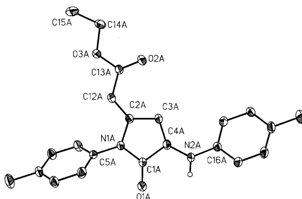
Figure 1. ORTEP plot of 3c . The thermal ellipsoids of 50% probability are shown for the non-hydrogen atoms; selected bond lengths (Å) and angles (°): O(1)–C(1) 1.212(5), N(1A)–C(1A) 1.371(5), C(2A)–C(12A) 1.342(5), N(1A)–C(2A) 1.414(5), C(2A)–C(3A) 1.450(5), C(1A)–C(4A) 1.504(5); C(1A)–N(1A)–C(5A) 124.2(3), O(1A)–C(1A)–C(4A) 127.5(3), N(1A)–C(1A)–C(4A) 106.0(3), C(4A)–C(3A)–C(2A) 108.4(3)
