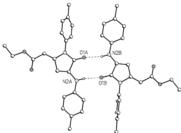
Figure 2. Dimeric structure of 3c
