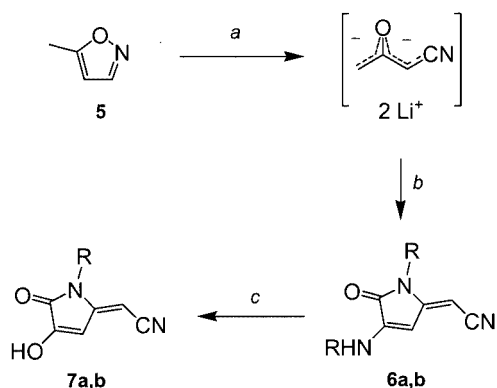
Scheme 5. Synthesis of 5-alkylidene-2,5-dihydropyrrol-2-ones 7a,b . a: 2.2 equiv. LDA [ 6a (R = Tol), 44%; 6b (R = Ph), 40%]; b: 2b,c , THF, –78 to 20 °C; c: 1 M HCl, THF, 1 h, 20 °C [ 7a (R = Tol), 63%; 7b (R = Ph), 52%]
