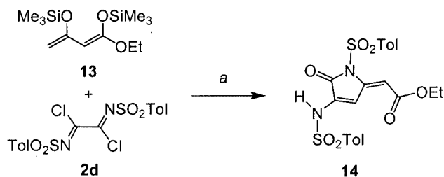
Scheme 9. Lewis acid-mediated cyclization of 1,3-bis(silyl enol ether) 13 with 2d , a: 2.0 equiv. \text{TiCl}_4 , \text{CH}_2\text{Cl}_2 , -78 to 20 °C, 15%
