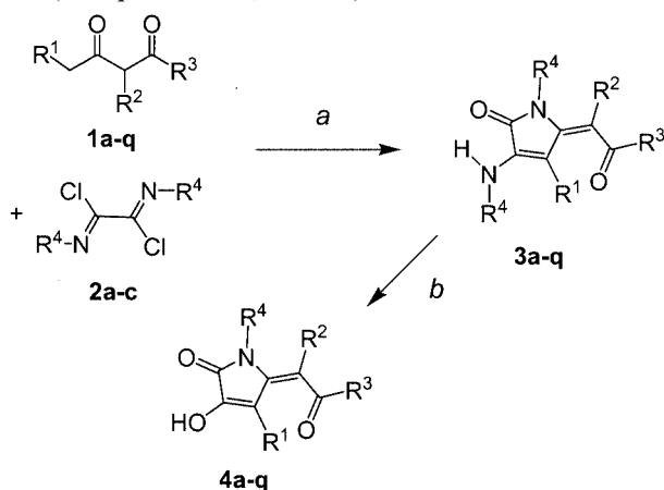
Scheme 4. Synthesis of 5-alkylidene-2,5-dihydropyrrol-2-ones 4a–q , a: 1) 2.2 equiv. LDA, 2) 2a–c , THF, –78 to 20 °C; b: 1 M HCl, THF, 1 h, 20 °C.
