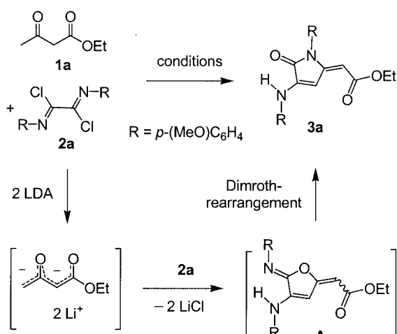
Scheme 2. Mechanism of the formation of 3a . Conditions: 1) 2.2 equiv. LDA, 2) 2a , THF, -78 then 20 °C, 56%
