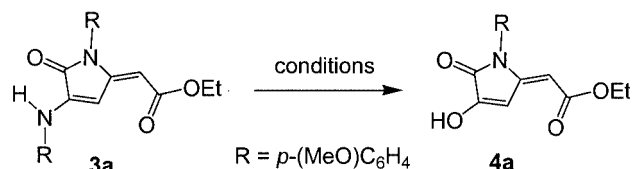
Scheme 3. Hydrolytic cleavage of the enamine moiety 3a . For conditions see Table 1.
