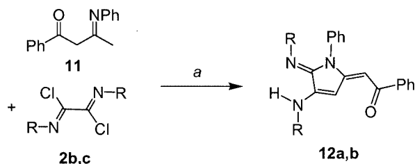
Scheme 8. Cyclization of dilithiated 11 with 2b,c : a: 1) 2.2 equiv. LDA, 2) 2b,c , THF, -78 to 20 °C [ 12a (R = Tol), 35%; 12b (R = Ph), 32%].
