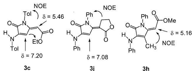
Scheme 6. Chemical shifts and NOESY experiments
