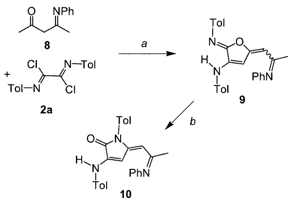
Scheme 7. Cyclization of dilithiated 8 with 2c : a) 1) 2.2 equiv. LDA, 2) 2c , THF, -78 to 20 °C, 45% [( E )/( Z ) = 1:1, the product contains ca. 20% of an unknown isomer]; b) THF, 72 h, 20 °C, 12% (low conversion); alternatively: THF, LiCl, 72 h, 56%.
